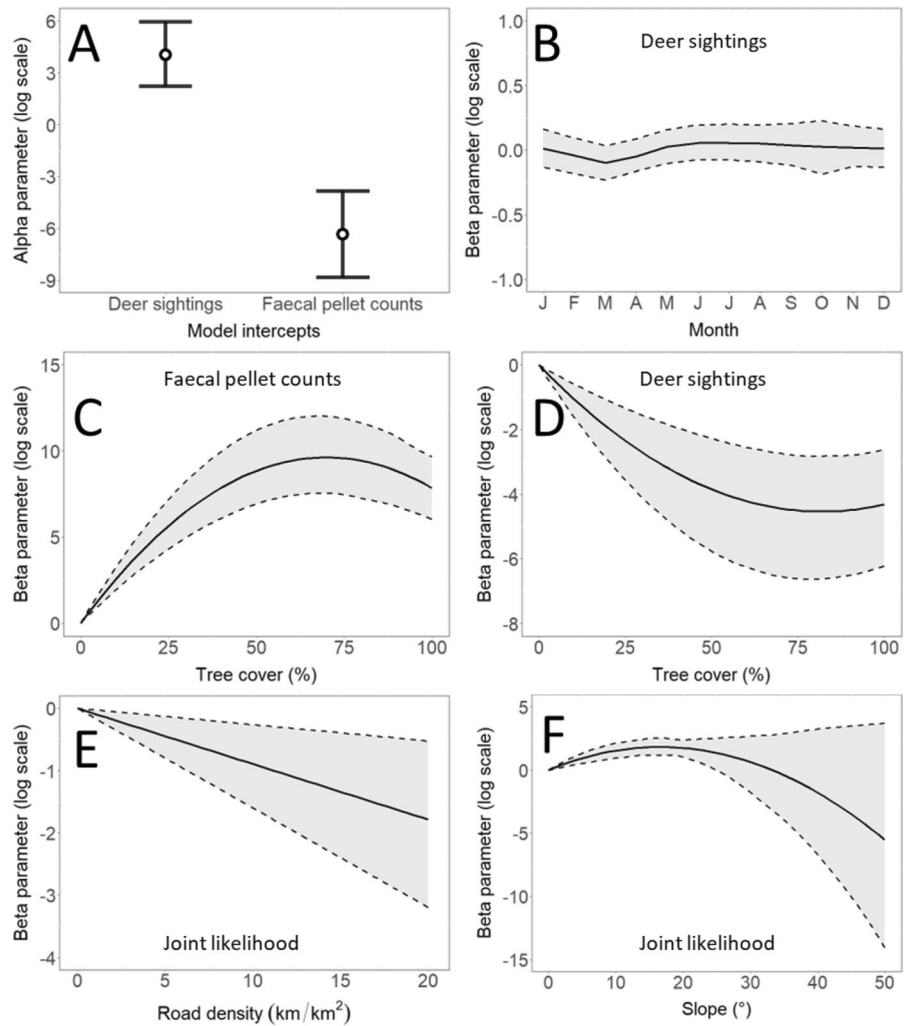
Fig. 4 Mean effects (solid lines) and 95% credible intervals (dashed lines) of spatio-temporal variables on faecal pellet counts and deer sightings during the Illawarra Wild Deer Management Program in the Wollongong LGA, eastern Australia, 2011–2021. All effects (alpha and beta parameters) are shown on the link-scale (i.e., log scale for negative binomial regressions), see Materials and methods for the full joint likelihood model formula. A Intercepts (alpha parameters) for the two sub-models of our joint likelihood model; B effect (beta parameter) of month on deer sightings; C effect of tree cover on faecal pellet counts; D effect of tree cover on deer sightings; E effect of road density on both faecal pellet counts and deer sightings (i.e., joint likelihood); F effect of slope on both faecal pellet counts and deer sightings
