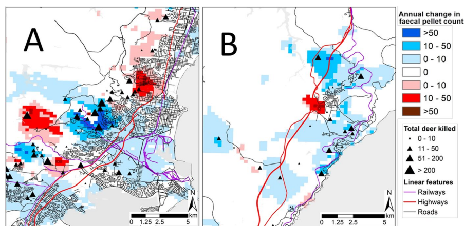
Fig. 6 Expected annual change in faecal pellet counts and cumulative vehicle-based professional shooting of rusa deer during the Illawarra Wild Deer Management Program in the Wollongong LGA, eastern Australia, 2011–2021. Blue=decrease (negative linear regression slopes with 95%
