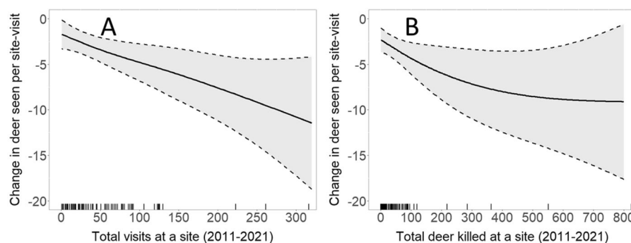
Fig. 7 Expected change in deer sighting with increasing site-visits (A) and total deer killed per site (B) from vehicle-based professional shooting of rusa deer during the Illawarra Wild Deer Management Program in the Wollongong LGA, eastern
